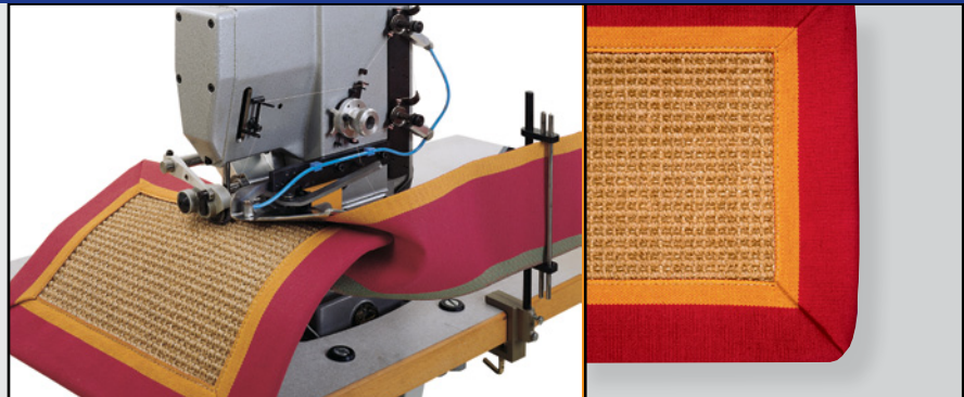
View of the TITAN DK 3700C sewing large tape of 150 mm width on a sisal carpet
